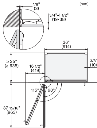
KFMC3642R, KFMC3642L, KFMC3844R, KFMC3844L, MasterCool III, panel ready, top view (installation drawing) (US)
