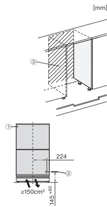
KU7175D, Built-under, installation drawing (*footnote)
