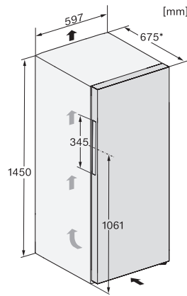
K4323FD, K4323ED, K4323DD, FN4322E, FN4322D, FN4322D ws-1, installation sketch
