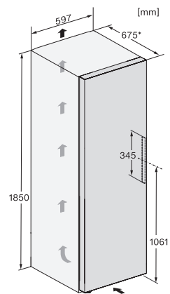
FNS4382D, FNS4382E, installation sketch
