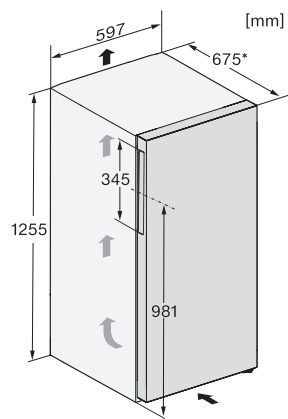
FN4312E, FN4312D, installation sketch
