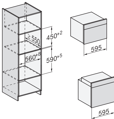
H226x-1B/BP/E/EP/I/IP, H2760B/BP, H28x0B/BP, H7x40BM/BMX, H7x6x6/BP/BPX, installation drawings
