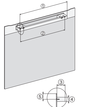
DG2840, DG7x40, DGC7x4x, DG7x6x, DGC7x6x, DGD7635, DGM7x4x, DO7, H28B/BP, H7x4xB/BM/BP, H7x6xB/BP, installation drawing
