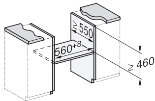
H2840B, H7244B, H7244BP, H7440B, H7440BPX, H7640BP, H7840BP, H7840BPX, installation drawings
