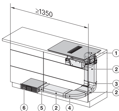
KMDA7676-1FL, KMDA7876-1FL, KMDA7676FL, KMDA7876FL – Installation variant 5 Circulating air
