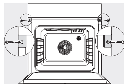
Installation_DGC_XXL_ESW7x10_EVST010 installation drawings
