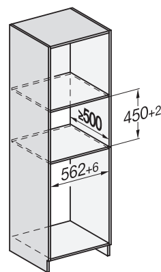
CVA7000 (installation drawings)
