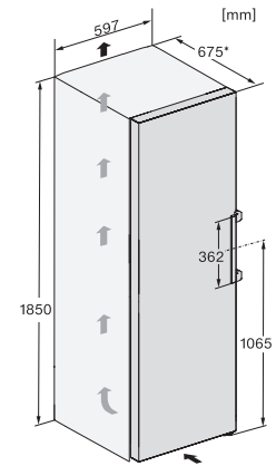
FNS4782E, FNS4782D, FNS4782E C, FNS4382E N, Nordic, installation sketch (footnote*) (installation drawings)
