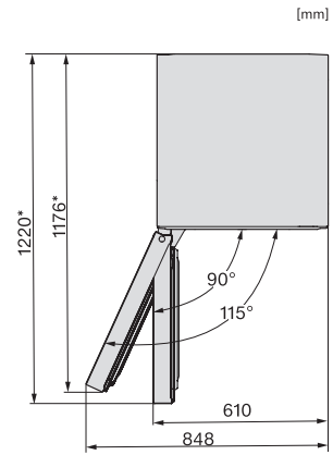
FNS4882D, top view (footnote*) (installation drawings)
