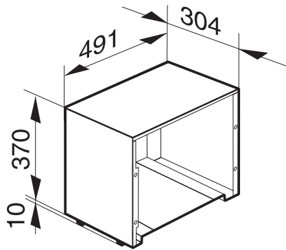
DGSG50 (installation drawing)
