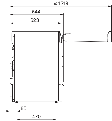
T2 with glass door, fascia 17 degree, with QuickPowerDry, measures in mm
