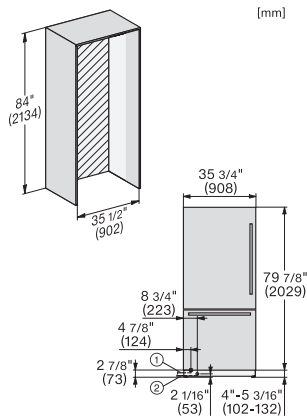
KFMC3642R + L, KFMC3844R + L, MasterCool III, PACS, with stainless steel front, installation
