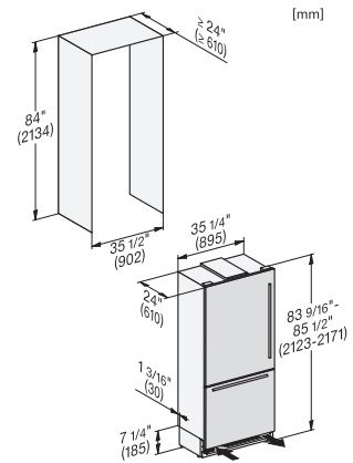
KFMC3642R, KFMC3642L, KFMC3844R, KFMC3844L, MasterCool III, PACS, with stainless steel front, integration
