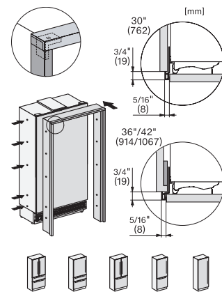
KFMC3632R+L, KFMC3642R+L, KFMC3836R+L, KFMC3834R+L, KFMC3858FD, MasterCool III, frame neutral, installation
