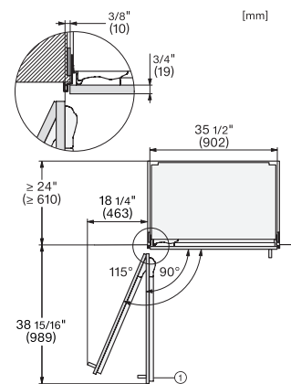
KFMC3642R, KFMC3642L, KFMC3844R, KFMC3844L, MasterCool III, PACS, with stainless steel front, top view
