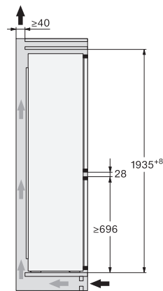
KFN7934D, side view
