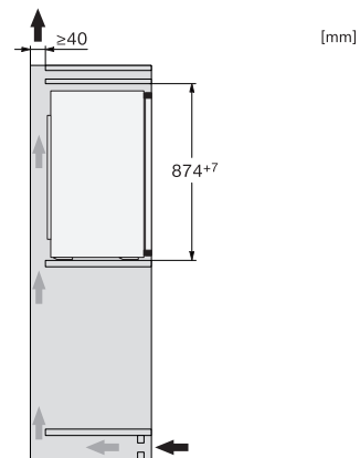
K7113D, K7113F, K7114E, K7103F, K7103D, K7104E, side view (installation drawings)
