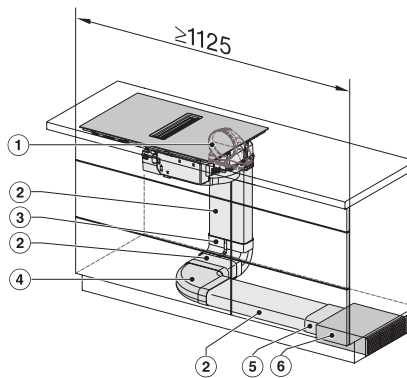
KMDA7272-1FL/FR, KMDA7473-1FL/FR, KMDA7272FL/FR, KMDA7473FL/FR – Installation variant 13 Circulating air
