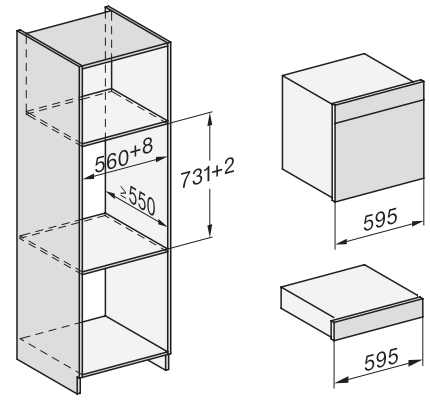
Installation_DGC_XXL_ESW7x10_EVS7010 installation drawings
