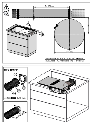
Installation plan DVS150PP
