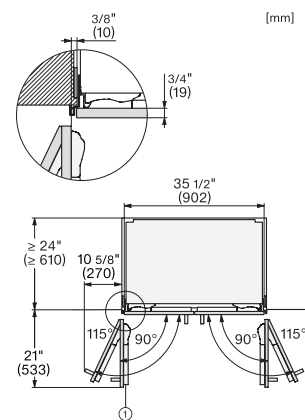
KFMC3642FD, KFMC3844FD, MasterCool III, PACS, with stainless steel front, top view
