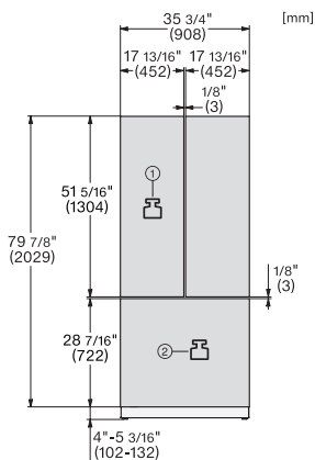
KFMC3642FD, KFMC3844FD, MasterCool III, front view
