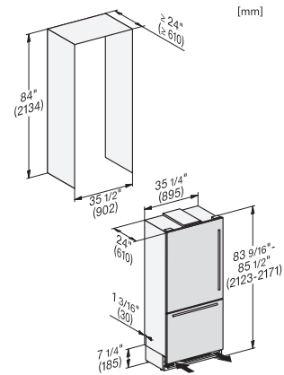
KFMC3642R, KFMC3642L, KFMC3844R, KFMC3844L, MasterCool III, PACS, with stainless steel front, integration
