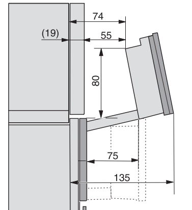
DGC7x4x swivel range of the aperture, installation drawings
