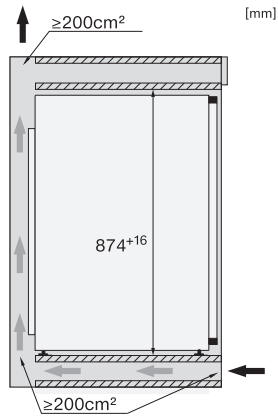
FNS7140B, FNS7140C, FNS7140D, FNS7140E, side view (installation drawings)
