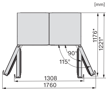
FNS4782E, FNS4782D, FNS4382D N, FNS4382E N, Nordic, installation (footnote*) (installation drawings)
