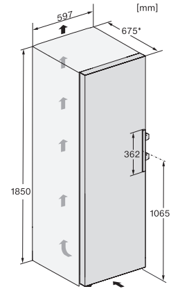
FNS4782E N, FNS4882D N, FNS4383E N, Nordics, installation sketch (footnote*) (installation drawings)
