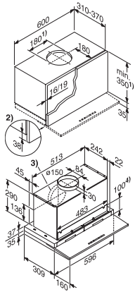
DA 3668 (installation drawing)
