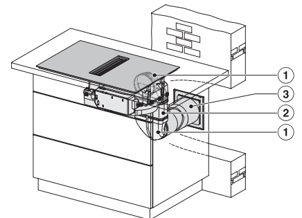
KMDA7676-1FL, KMDA7876-1FL, KMDA7676FL, KMDA7876FL – Installation variant 5 Circulating air
