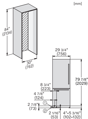
KFMC3632R+L, KFMC3836R+L, KFMC3834R+L, MasterCool III, PACS, stainless steel front, installation
