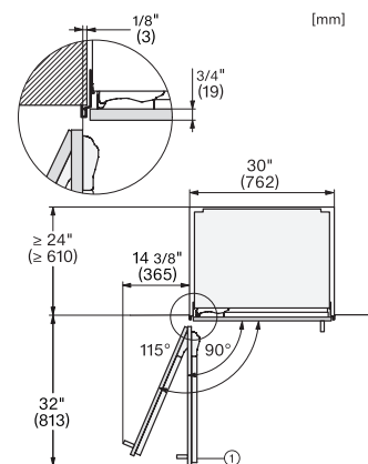
KFMC3632R+L, KFMC3836R+L, KFMC3834R+L, MasterCool III, PACS, with stainless steel front, top view
