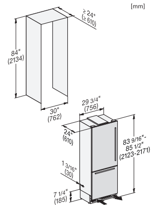
KFMC3632R+L, KFMC3836R+L, KFMC3834R+L, MasterCool III, PACS, with stainless steel front, integration
