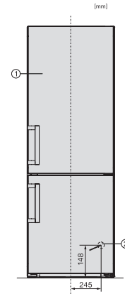
KFN4796AD, KFN4796CD, installation (footnote*) (installation drawings)
