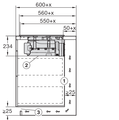
KMDA7676FL, KMDA7876FL – Side view lying on top+X, Plug&Play – Installation drawing
