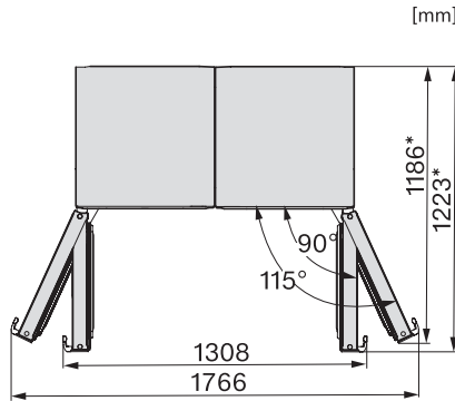
FNS4782E, FNS4782D, FNS4782E N, FNS4782D N, FNS4882D N, FNS4882E N, top view (footnote*) (installation drawings)
