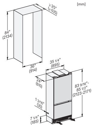
KFMC3642R, KFMC3642L, KFMC3844R, KFMC3844L, MasterCool III, Integration, panel ready, (Skizze)
