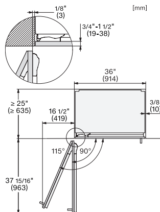
KFMC3642R, KFMC3642L, KFMC3844R, KFMC3844L, MasterCool III, panel ready, Draufsicht (Skizze)
