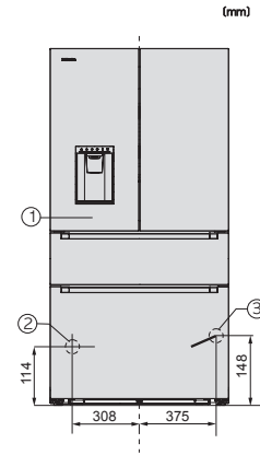
E-Com, KFFD6765 edt/cs, Installation (*Fußnote)
