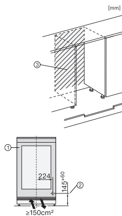
KWTUS7054F, KWTUS7055F, KWTUS7074F, KWTUS7096E, KWTUS7196E, Built-under, Installationsskizze
