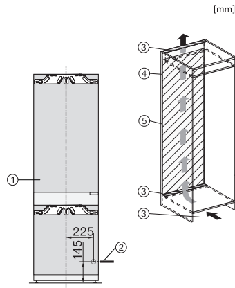
K7731F, K7731E, K7741F, Installation
