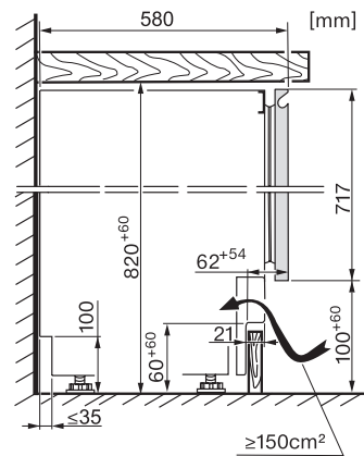
KWTUS7054F, KWTUS7055F, KWTUS7074F, Built-under, side view
