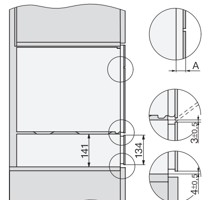
Side view_DG_DGM_ESW7x10_EVS7010 installation drawings
