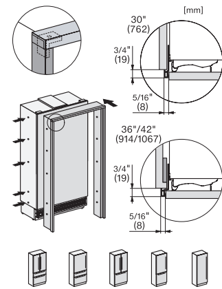
KFMC3632R+L, KFMC3642R+L, KFMC3836R+L, KFMC3834R+L, KFMC3846R+L, KFMC3858FD, MasterCool III, Rahmen neutral (Skizze)
