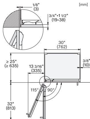
KFMC3632R+L, KFMC3836R+L, KFMC3834R+L, MasterCool III, panel ready, Draufsicht (Skizze)
