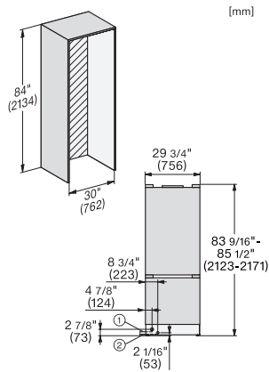
KFMC3632R+L, KFMC3836R+L, KFMC3834R+L, MasterCool III, Installation, panel ready (*Fußnote) (Skizze)
