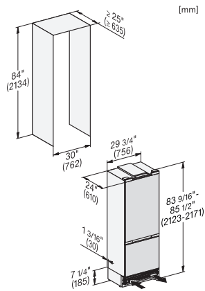
KFMC3632R, KFMC3632L, KFMC3836R, KFMC3836L, KFMC3834R, KFMC3834L, MasterCool III, Integration, panel ready, (Skizze)
