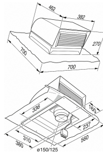
DDG102 (skiss)
