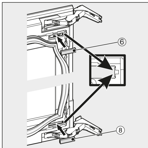
■ Refit covers ⑥ and ⑧.
