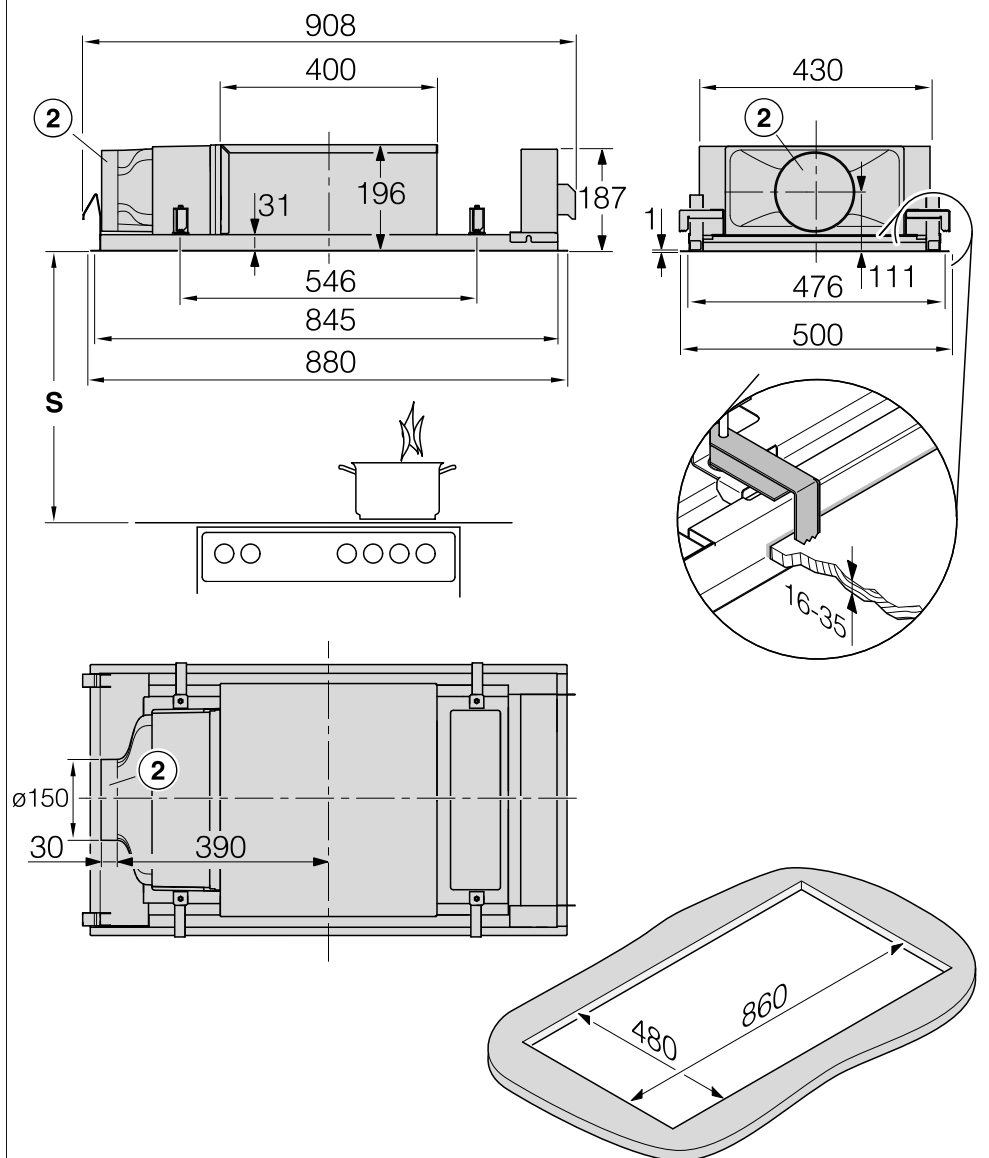
DAC 4940 in recirculation mode and Plug&Play recirculation mode
